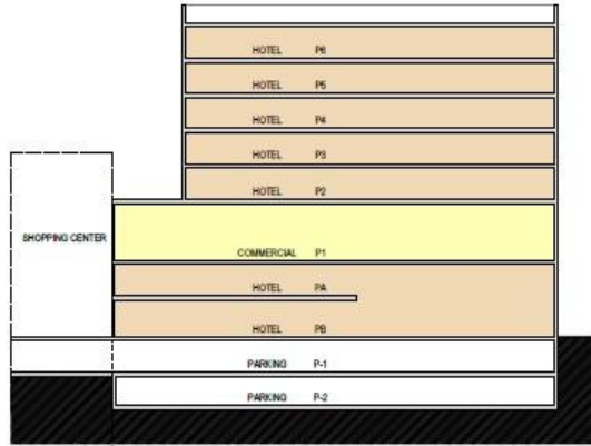
SECTION B-B
